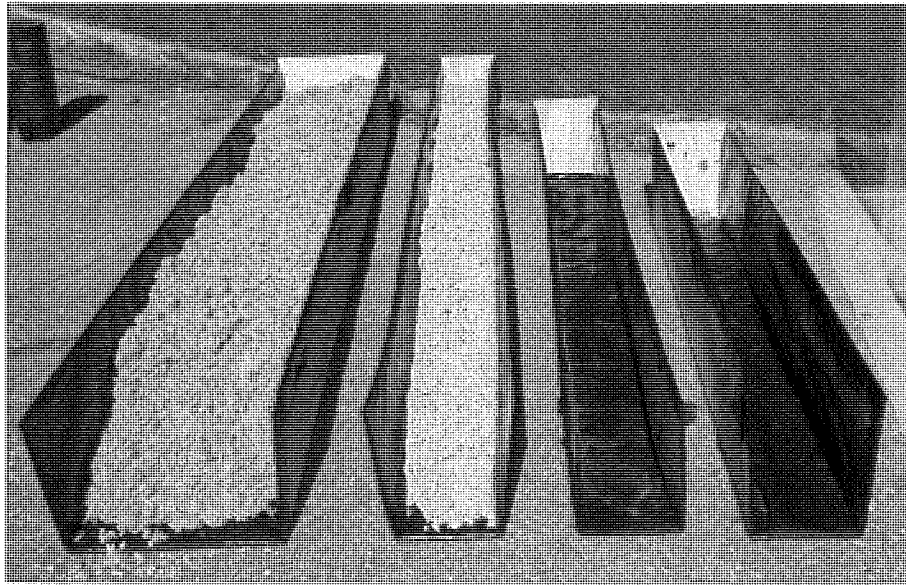
Illustration 1. Testing Chutes
